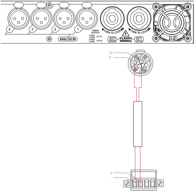
Figure 4.5: Bias Q5
