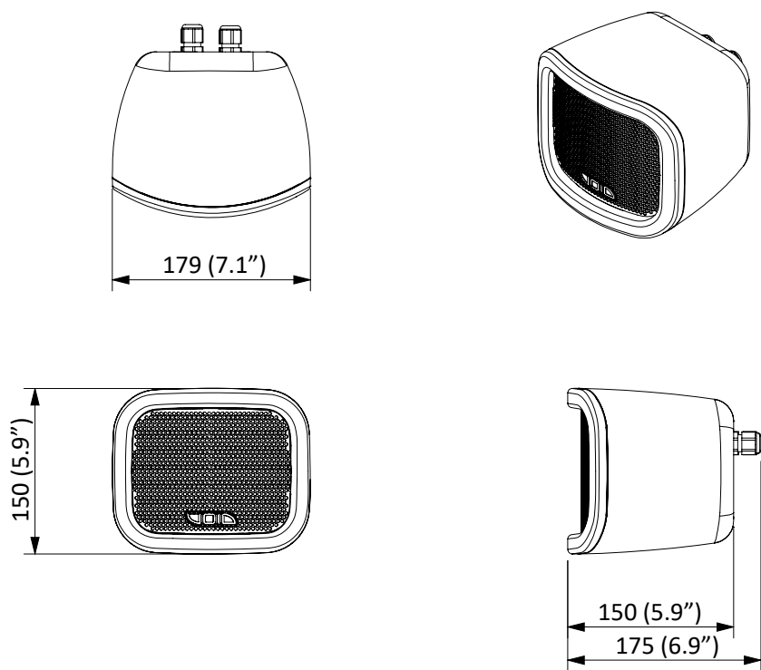
Figure 3.3: Dimensions
